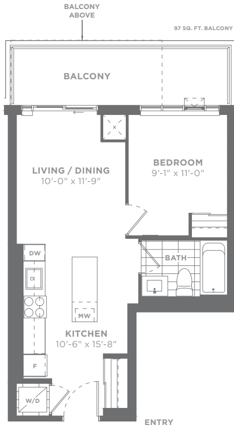
2 ND FLOOR
