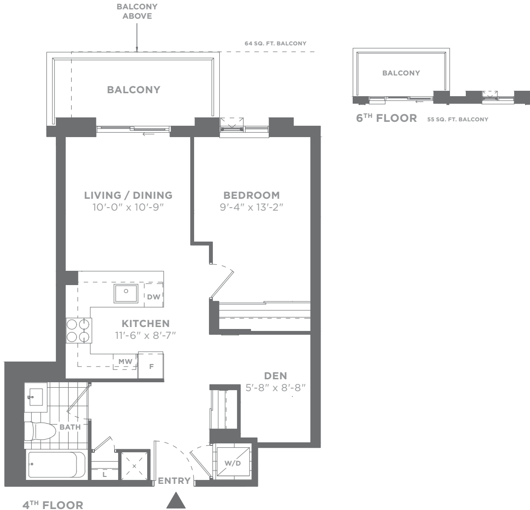
4 TH FLOOR
