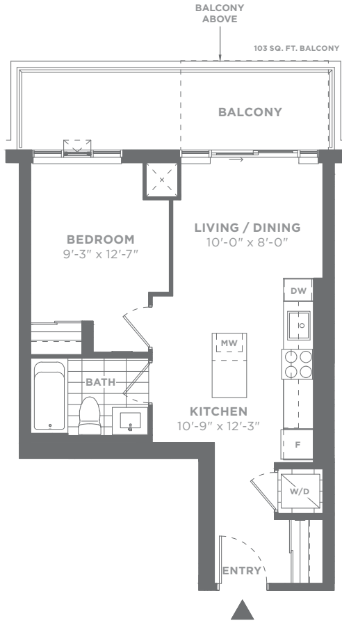
2 ND FLOOR
